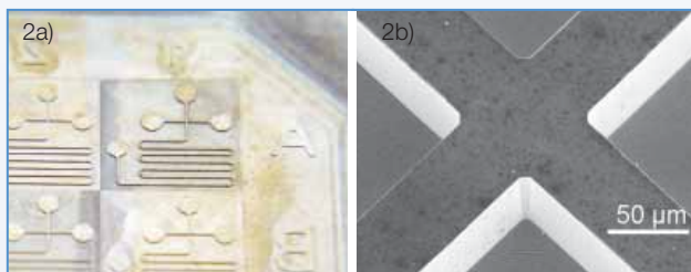
Figure 2a: Mould insert made of brass, manufactured by micro-milling.
