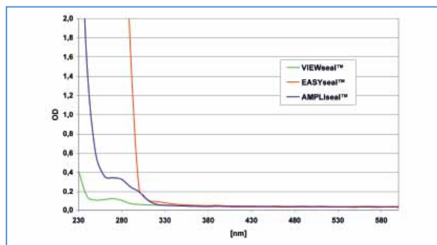
Figure 6: Light absorption of VIEWseal™, EASYseal™ and AMPLIseal™
