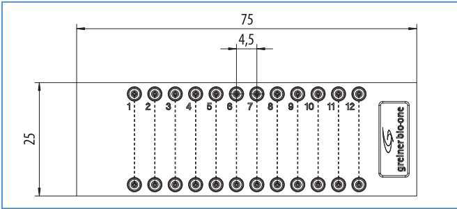
Figure 14: Schematic drawing of CrystalSlide™
