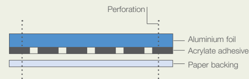
Figure 1: Structure of SILVERseal™
