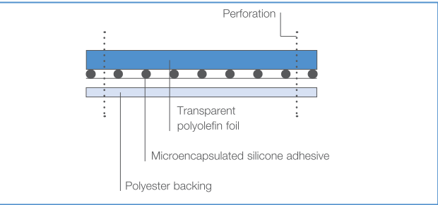
Figure 2: Structure of VIEWseal™
