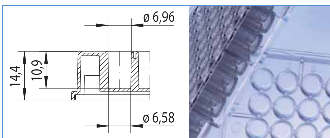
Figure 4: Well profile: 96 well F-bottom / chimney well, polystyrene Total volume: 392 µl Working volume: 25 – 340 µl Growth area: 34 mm²
